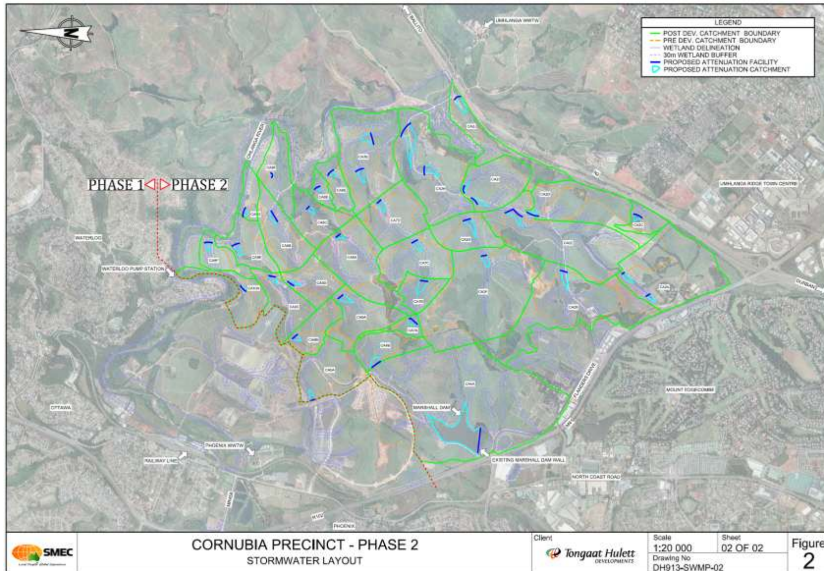
Figure 7-18: Proposed stormwater attenuation facilities within wetlands – Option 1
