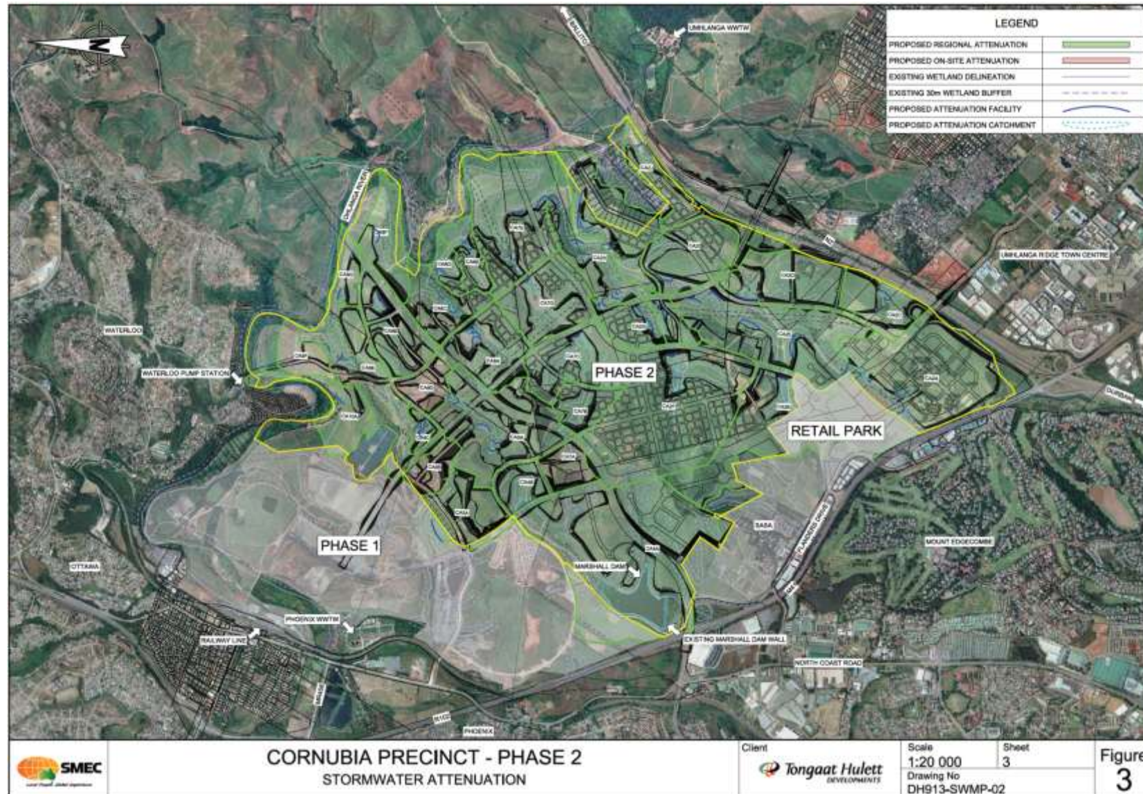
Figure 7-19: Proposed stormwater attenuation facilities within wetlands and outside of wetlands – Option 2
