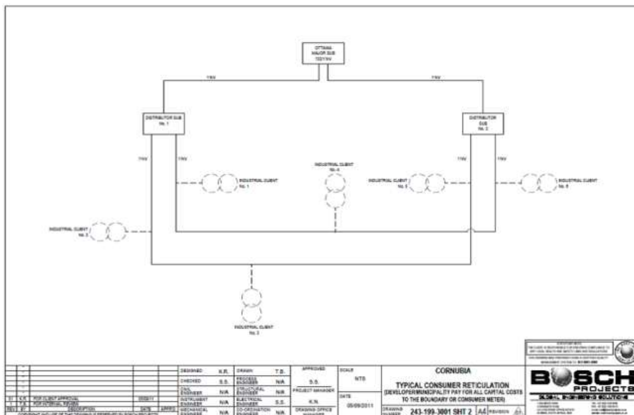
Figure 5-32: Typical consumer reticulation
