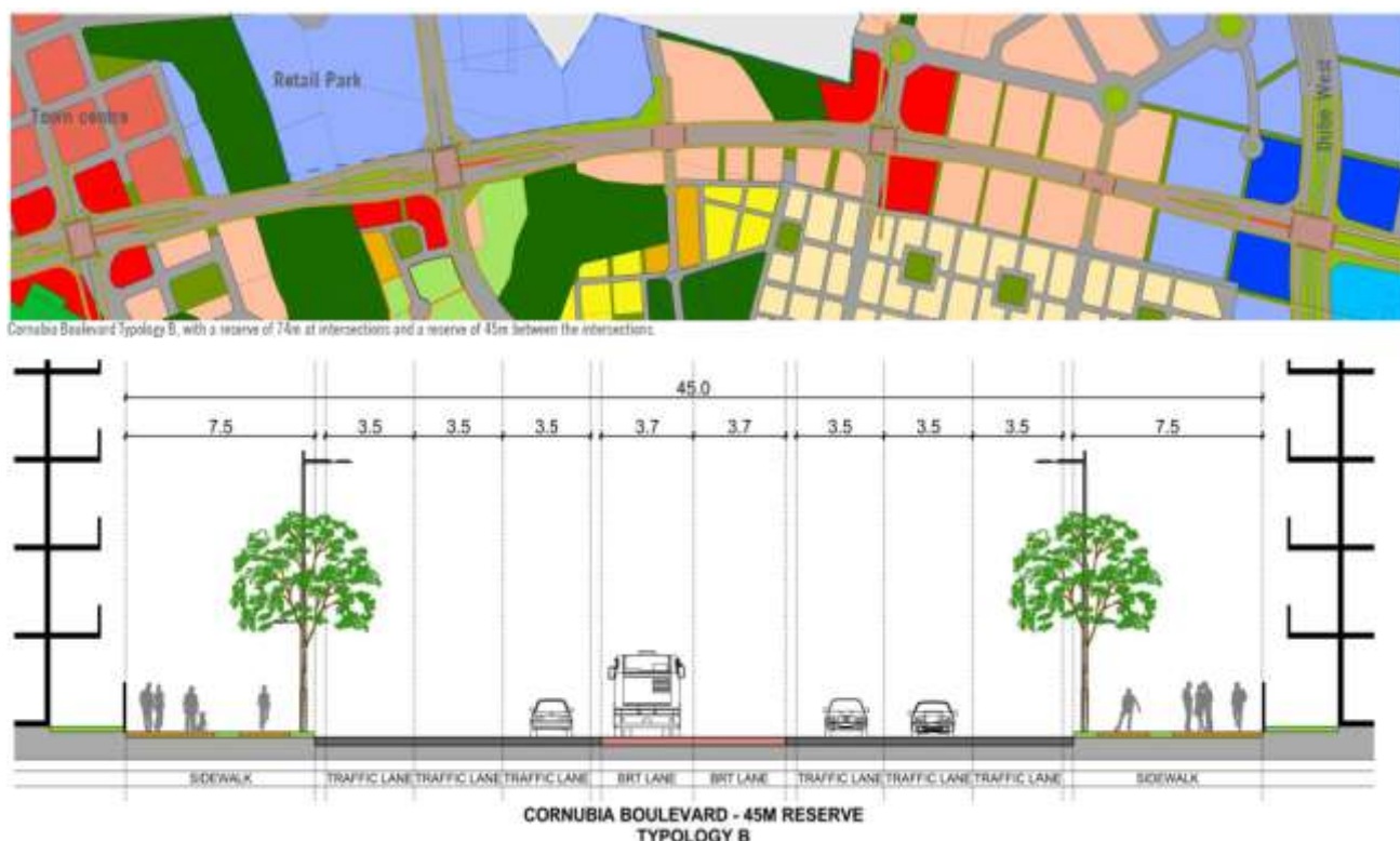
Figure 5-6: Cornubia Boulevard mobility structure – Typology B
